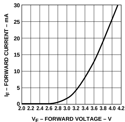
Figure 3. Forward current vs. forward voltage for devices with 3.8 V typical V_f .
