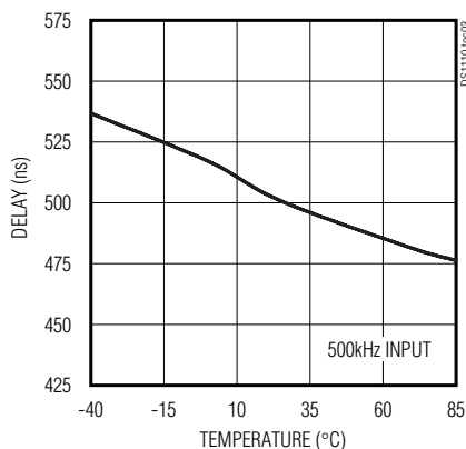
DS1110-500 TAP 10 DELAY vs. TEMPERATURE
