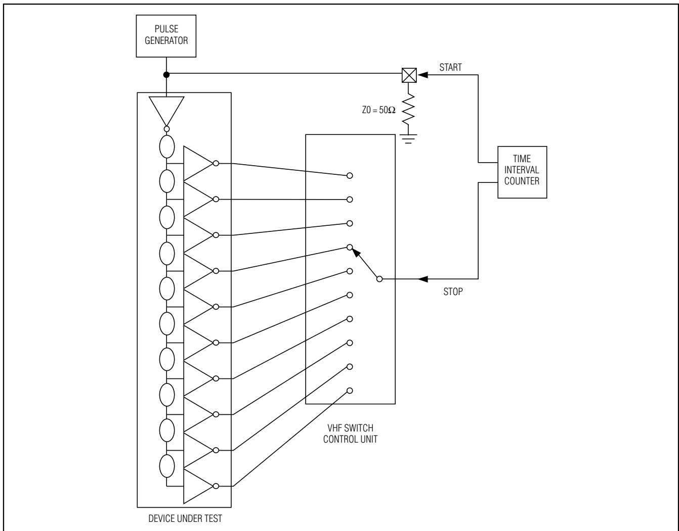
Figure 3. Test Circuit
