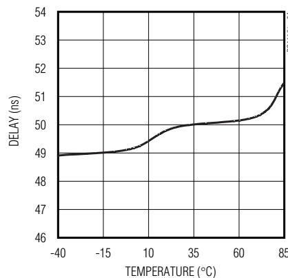
DS1110-50 TAP 10 DELAY vs. TEMPERATURE
