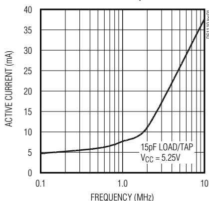
DS1110-500 ACTIVE CURRENT vs. INPUT FREQUENCY
