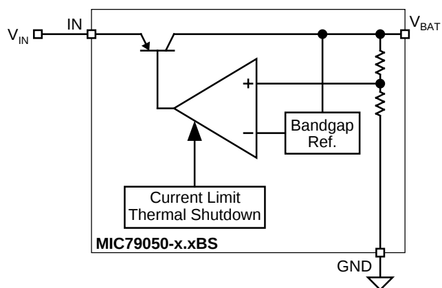
3-Pin Version
