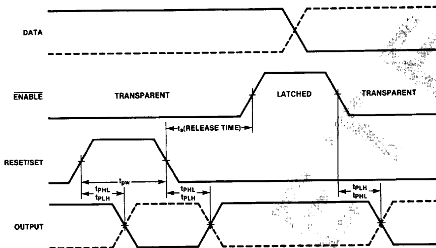
FIGURE 3. Reset Timing
