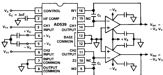
Figure 2. Standard Dual-Channel Multiplier
