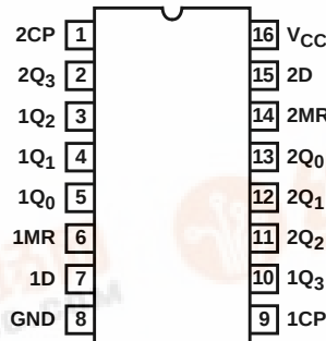
CD54HC4015 (CERDIP) CD74HC4015 (PDIP, SOIC) TOP VIEW
