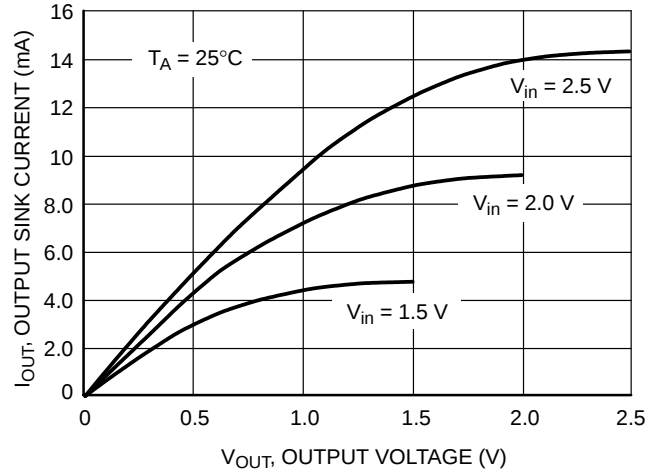
Figure 10. NCP300H/1L Series 2.7 V Reset Output Sink Current versus Output Voltage
