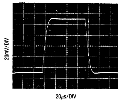
Small Signal Transient Response G = 10, V_S = \pm 15\text{V}
