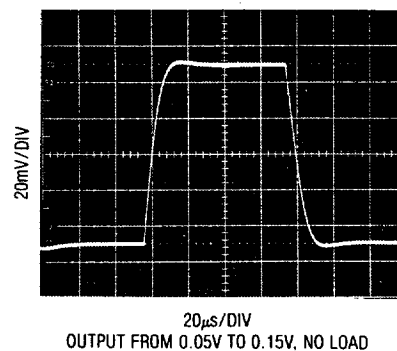
Small Signal Transient Response G = 10, V_S = 5\text{V}, 0\text{V}
