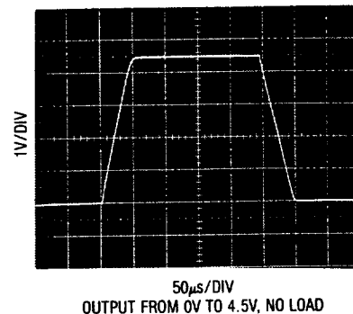
Large Signal Transient Response G = 10, V_S = 5\text{V}, 0\text{V}
