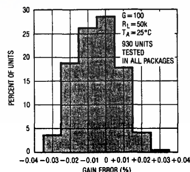
Gain Error Distribution
