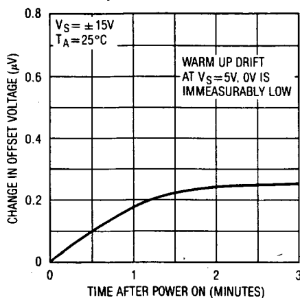
Warm-Up Drift
