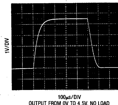
Large Signal Transient Response G = 100, V_S = 5\text{V}, 0\text{V}
