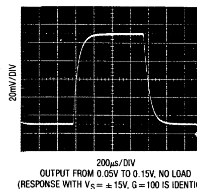
Small Signal Transient Response G = 100, V_S = 5\text{V}, 0\text{V}
