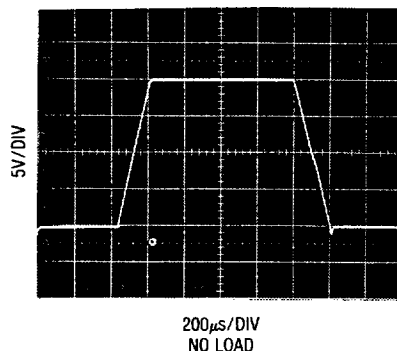
Large Signal Transient Response G = 10, V_S = \pm 15\text{V}
