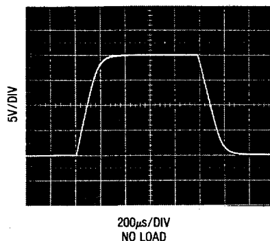
Large Signal Transient Response G = 100, V_S = \pm 15\text{V}
