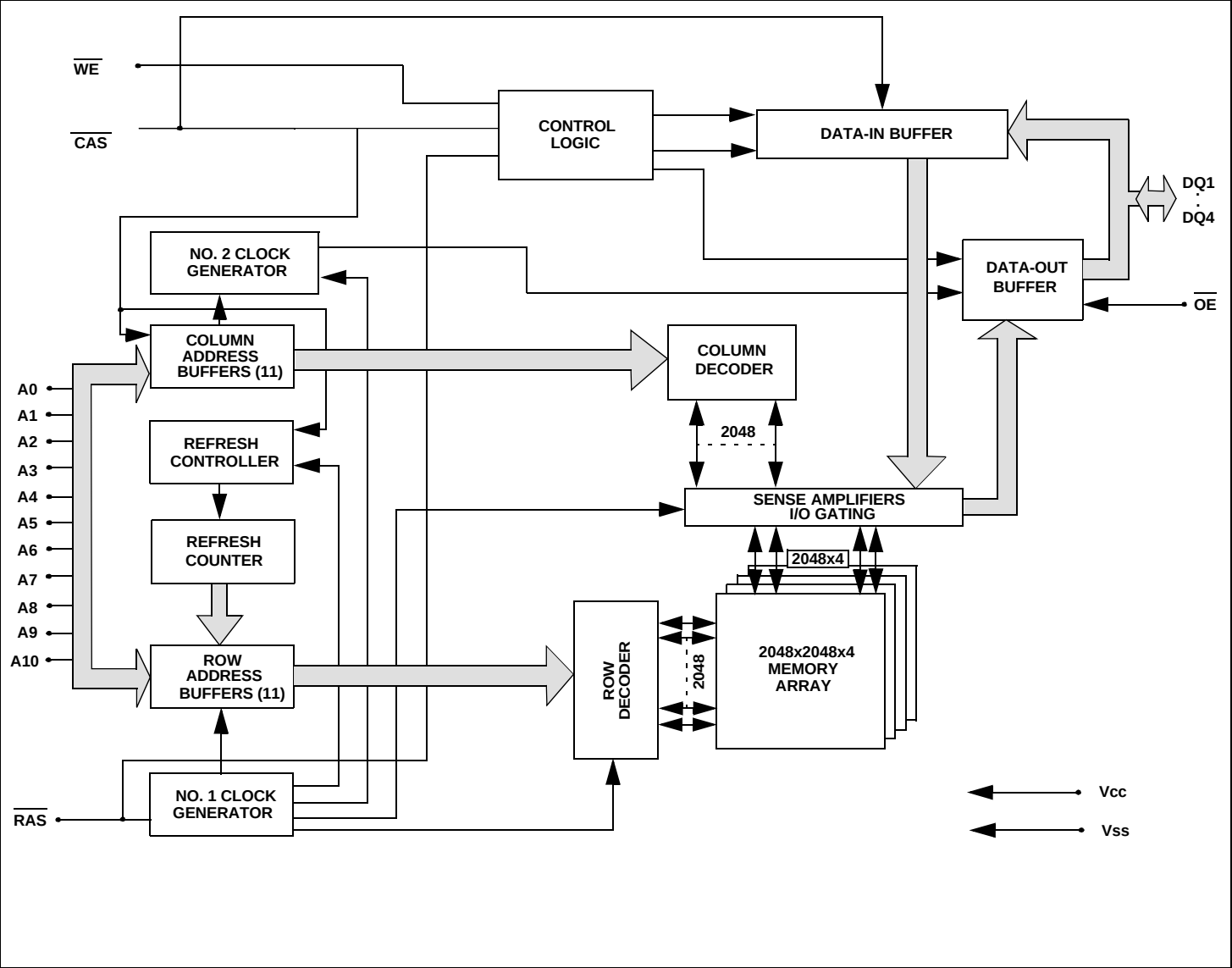
Block Diagram
