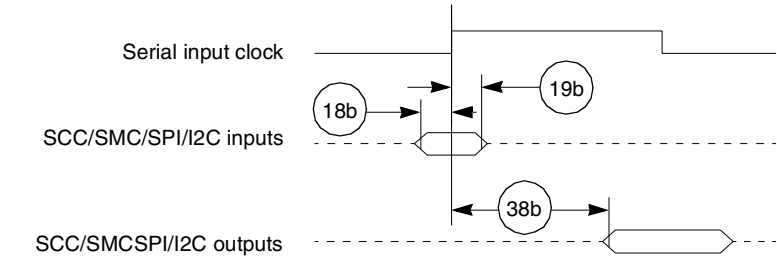
Figure 2-17. SCC/SMC/SPI/I 2 C External Clock Diagram
