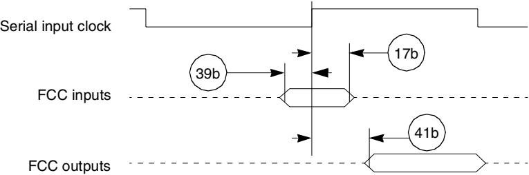
Figure 2-15. FCC External Clock Diagram
