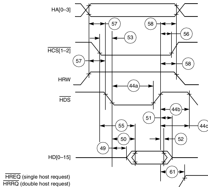
Figure 2-8. Read Timing Diagram, Single Data Strobe
