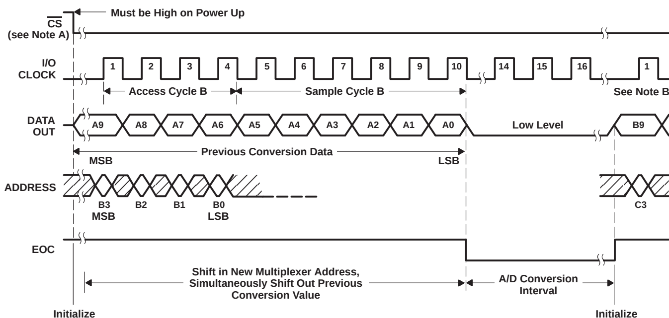
Figure 11. Timing for 11- to 16-Clock Transfer Using \overline{\text{CS}} (Serial Transfer Interval Shorter Than Conversion)
