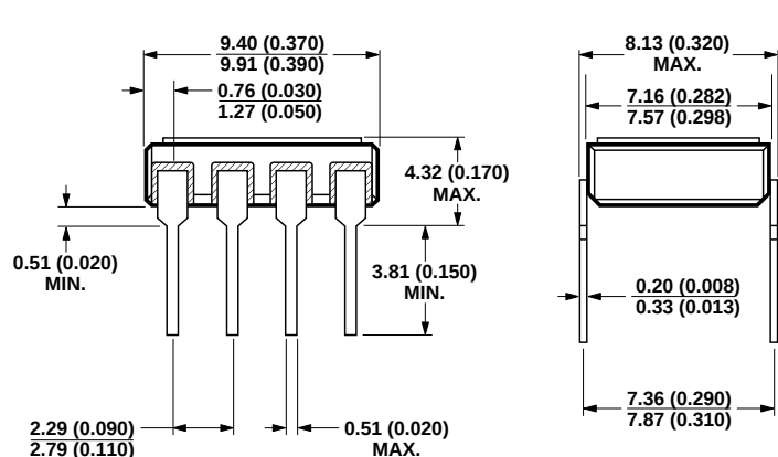
8 Pin DIP Through Hole, 1 and 2 Channel
