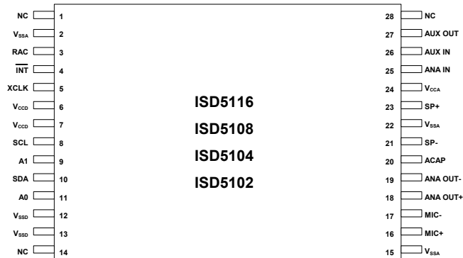
TSOP
