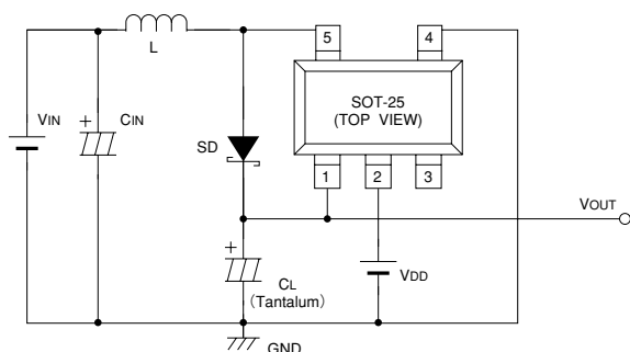
Fig.2 XC6381C Application
