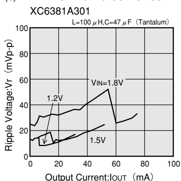
(3) RIPPLE VOLTAGE vs. OUTPUT CURRENT
