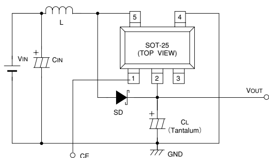
Fig.1 XC6381A Application
