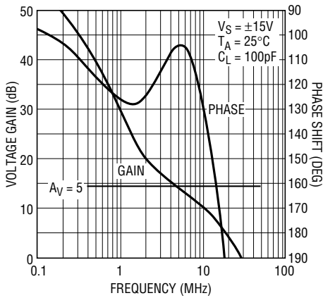
LT1037 Gain, Phase Shift vs Frequency
