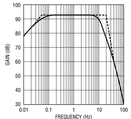
Figure 5b. 0.1Hz to 10Hz Peak-to-Peak Noise Tester Frequency Response
