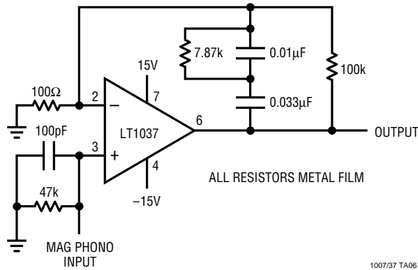
Phono Preampifier
