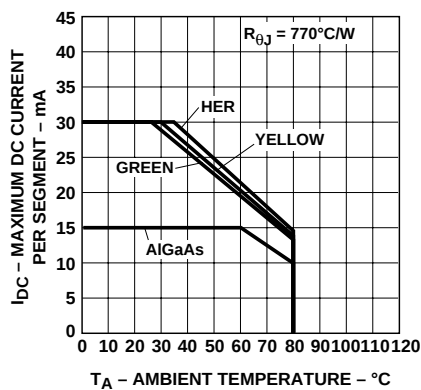
Figure 4. Maximum allowable DC current vs. ambient temperature.
