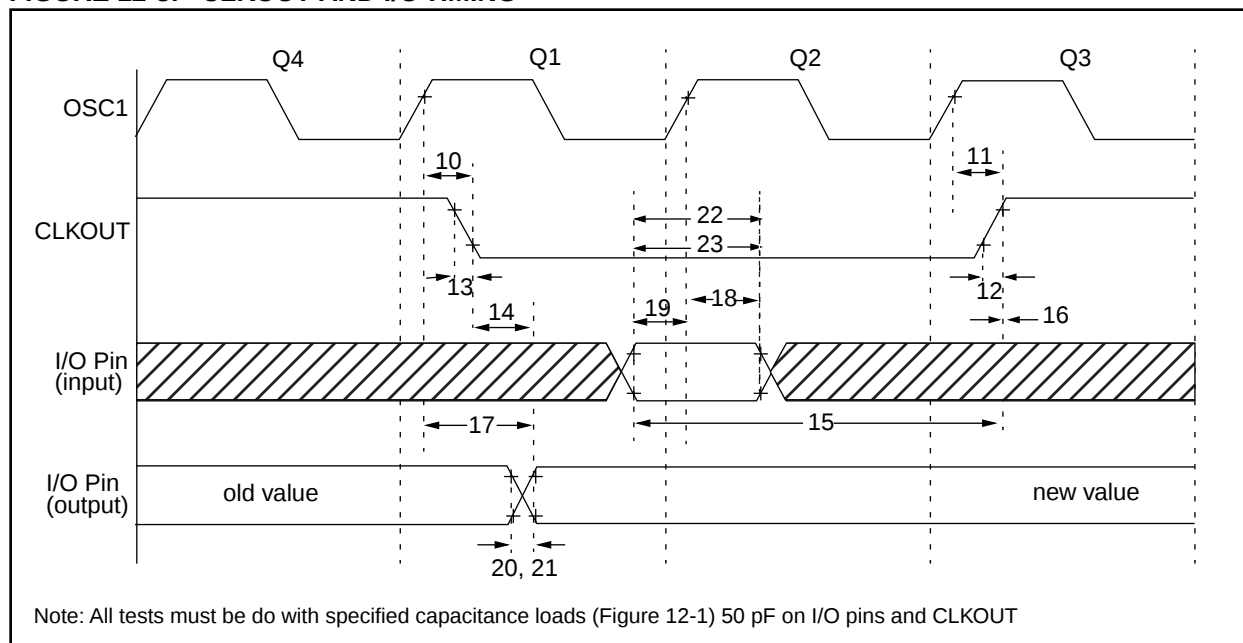
FIGURE 12-3: CLKOUT AND I/O TIMING
