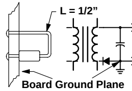
MOUNTING METHOD 3 P.C. Board with 1-1/2" x 1-1/2" Copper Surface
