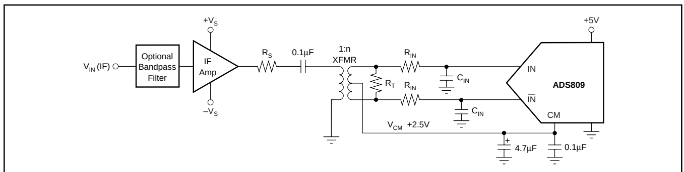
FIGURE 4. Driving the ADS809 with a Low-Distortion RF Amplifier and a Transformer Suited for IF Sampling Applications.
