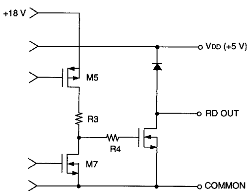
Figure 26. Relay Driver Output
