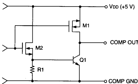
Figure 27. Comparator (Detector) Output
