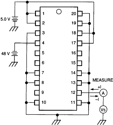
Figure 15. High-Voltage Leakage Current — Switch B
