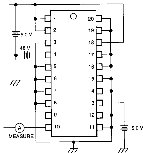
Figure 20. Relay Driver Output, Leakage Current
