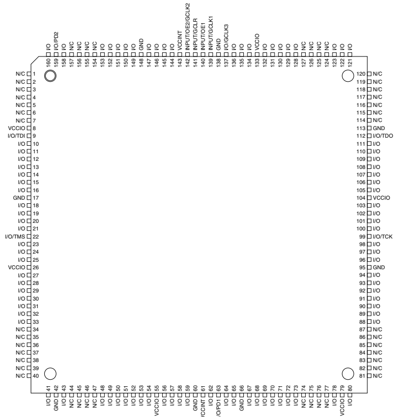
160-lead PQFP
