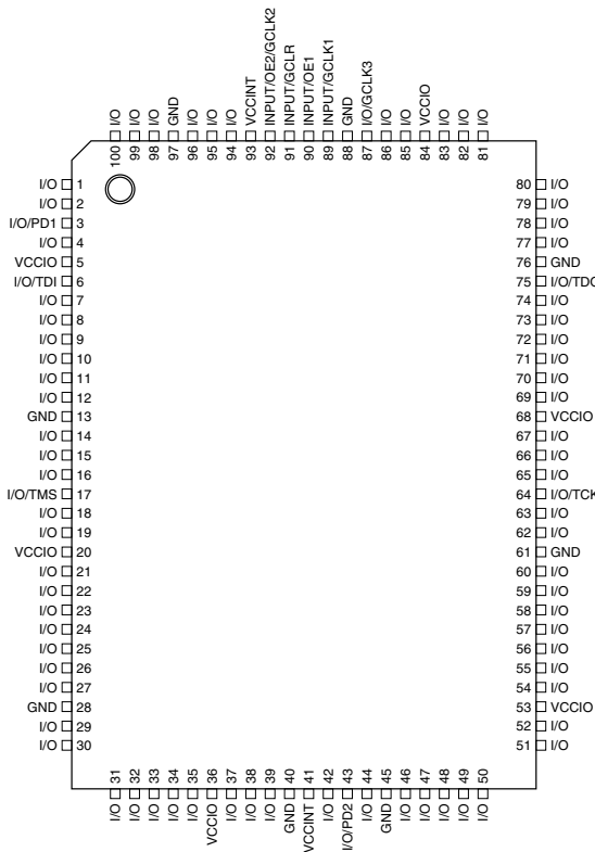
100-lead PQFP
