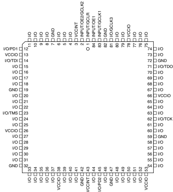
84-lead PLCC
