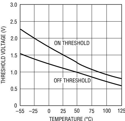
ON/OFF Thresholds
