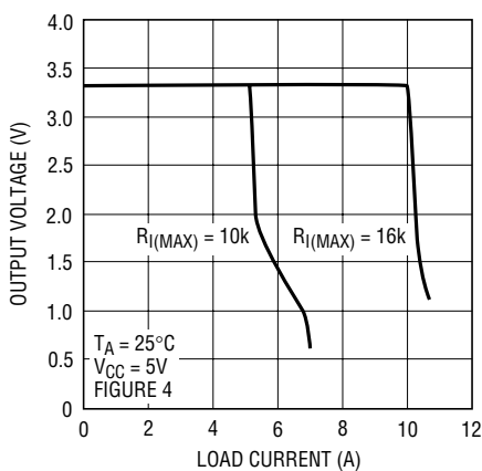
Output Voltage vs Load Current with Current Limit
