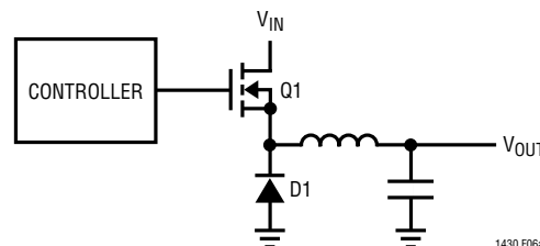
Figure 6a. Classical Buck Architecture
