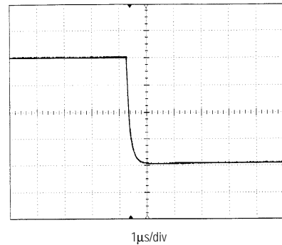
MAX520 NEGATIVE SETTLING TIME
