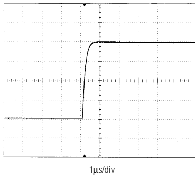
MAX520 POSITIVE SETTLING TIME
