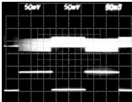
MAX730A LOAD-TRANSIENT RESPONSE
