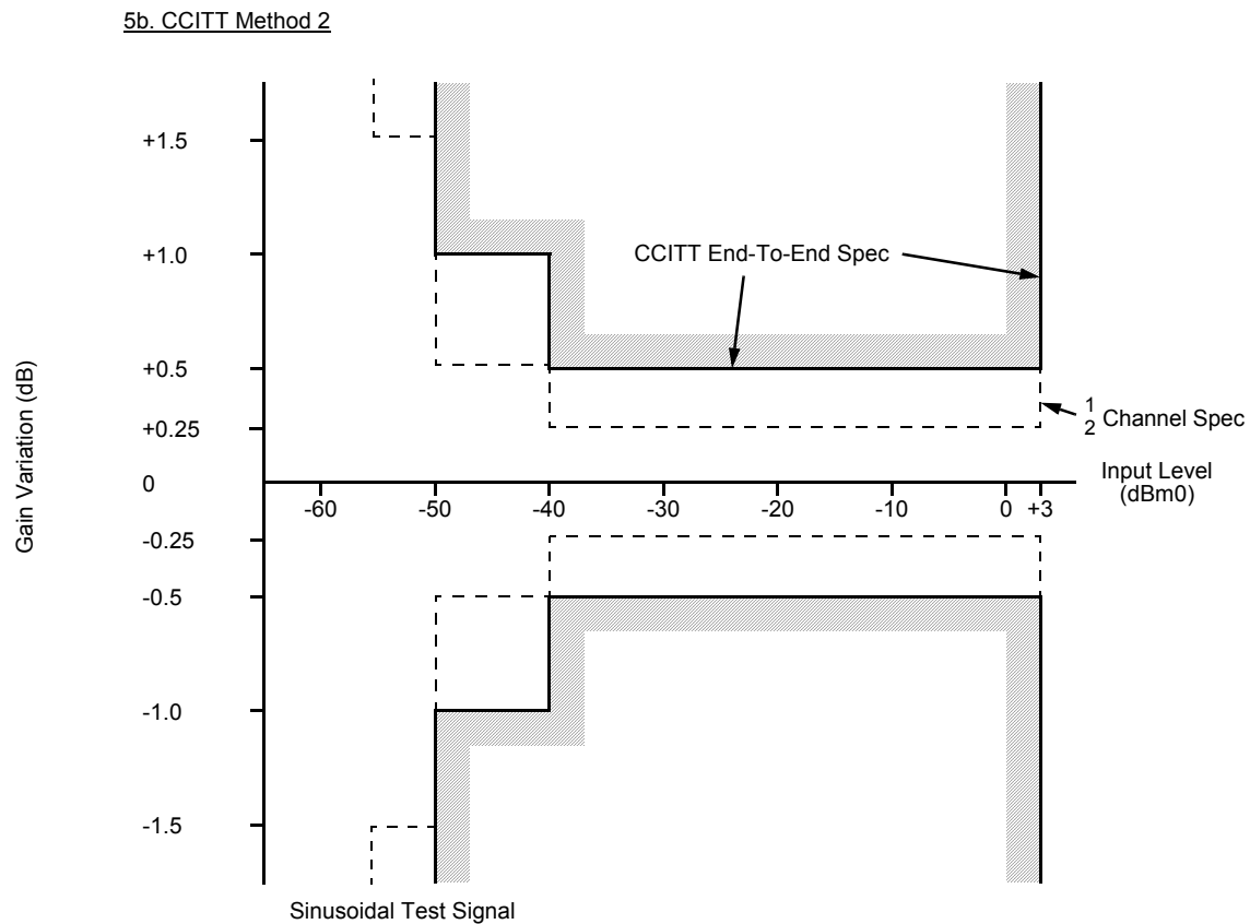
Figure 12 - Variation of Gain With Input Level
