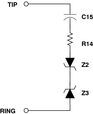
Figure 23. Ringer Impedance Network
