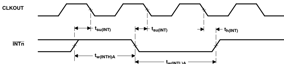
Figure 27. Interrupt Timing
