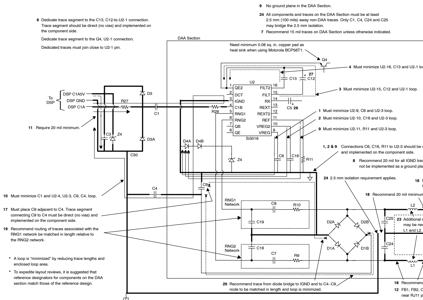
Figure 19. TMS320C54V90 Modem Layout Guidelines
