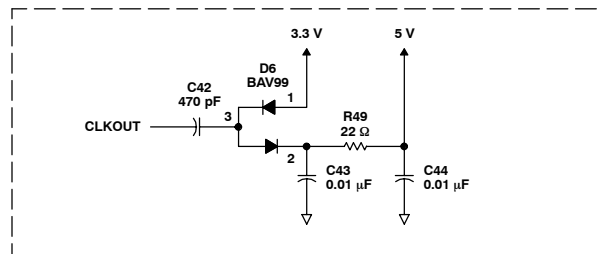
Optional 5 V Charge Pump†
