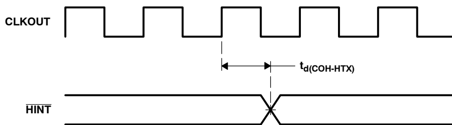
Figure 30. HINT Timing
