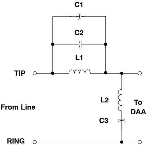
Figure 25. Dongle Applications Circuit
