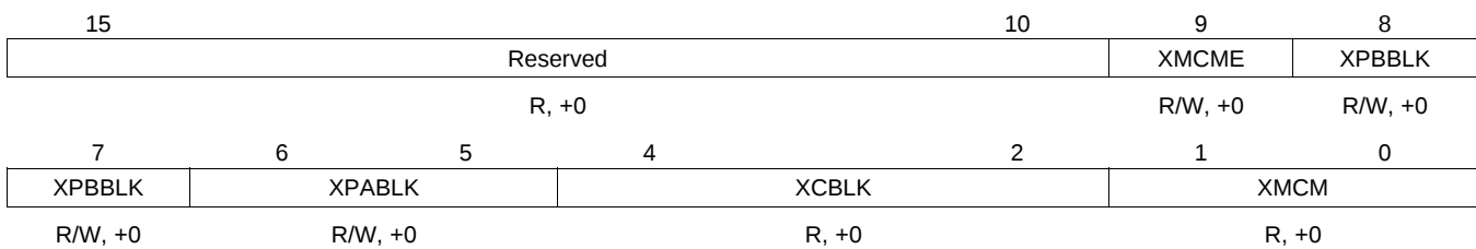
Figure 3-11. Multichannel Control Register 2x (MCR2x)
