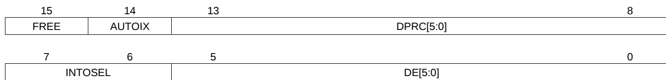
Figure 3-22. DMPREC Register
