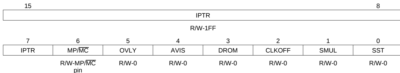
Figure 3-4. Processor Mode Status Register (PMST)
