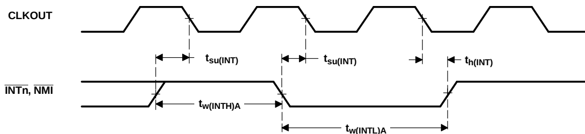
Figure 5-16. Interrupt Timing
