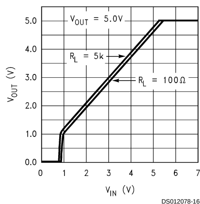
Dropout Characteristics
