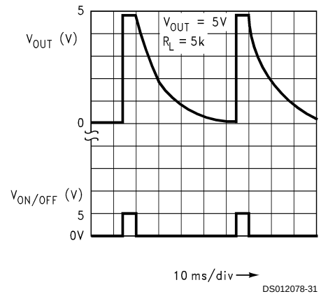
Turn-Off Waveform
