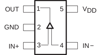
TLV2781 DBV PACKAGE (TOP VIEW)
