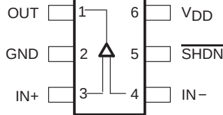
TLV2780 DBV PACKAGE (TOP VIEW)
