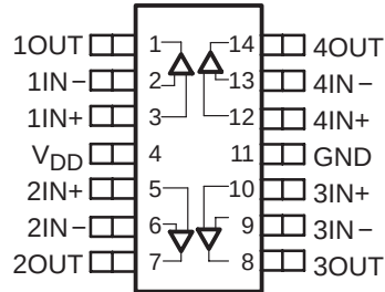
TLV2784 D, N, OR PW PACKAGE (TOP VIEW)
