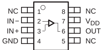
TLV2781 D OR P PACKAGE (TOP VIEW)
