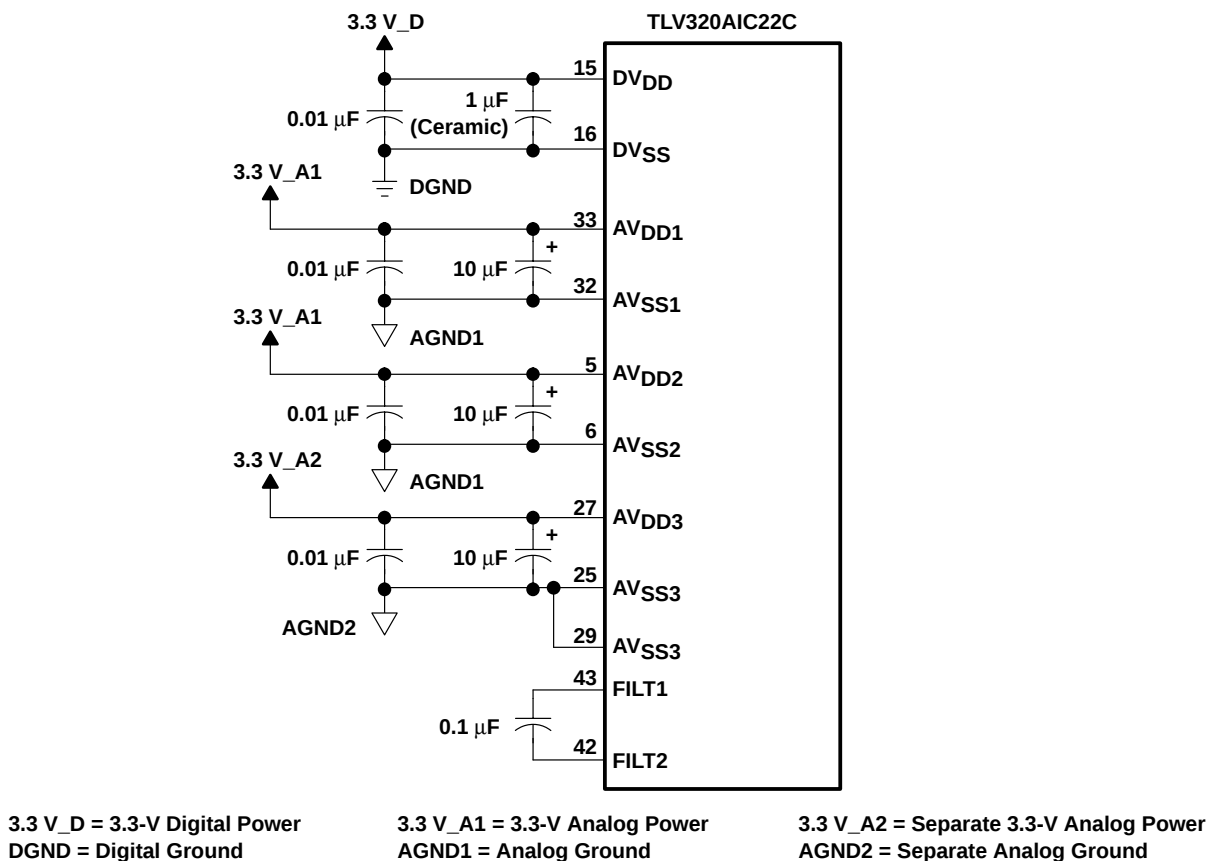
Figure 23. Recommended Decoupling
