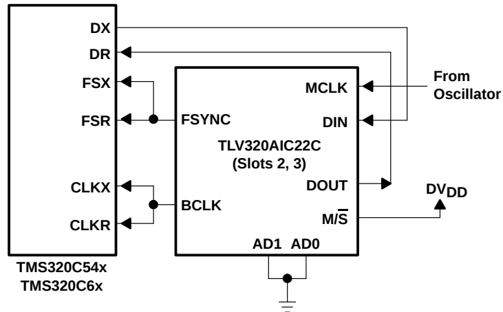
Figure 18. TLV320AIC22Cs Interface to McBSP Port of C54x or C6x DSP
