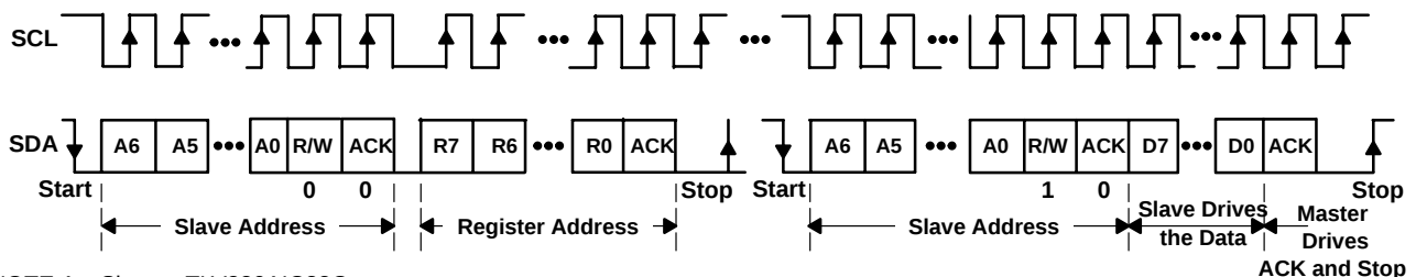
Figure 17. I 2 C Read From TLV320AIC22C (Protocol B)
