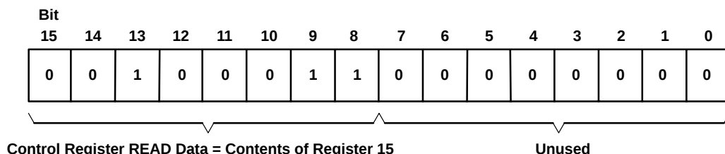
Figure 14. DOUT Data Stream for Programming Example 2, Slot 1
