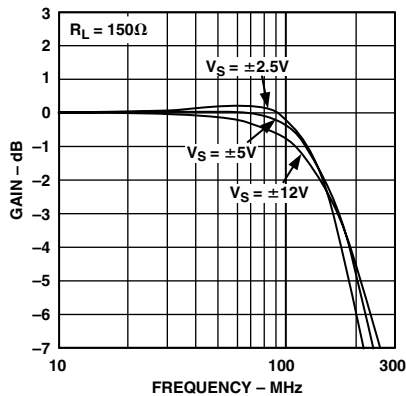
TPC 25. AD8129 Frequency Response vs. Supply, R_L = 150\text{ }\Omega
