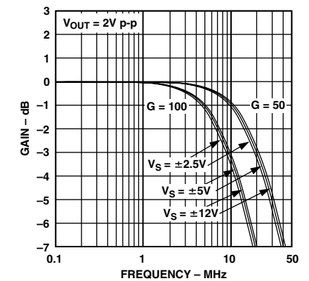
TPC 33. AD8129 Frequency Response vs. Supply, G = 50 , G = 100 , V_{OUT} = 2 \text{ V p-p}
