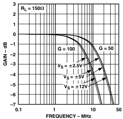
TPC 34. AD8129 Frequency Response vs. Supply, G = 50 , G = 100 , R_L = 150 \Omega
