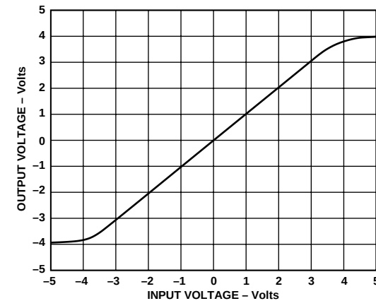
Figure 21. Output Voltage vs. Input Voltage, R_L = 1k\Omega
