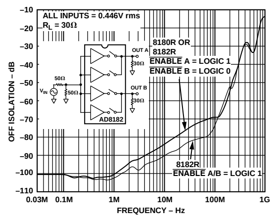
Figure 14. "OFF" Isolation vs. Frequency
