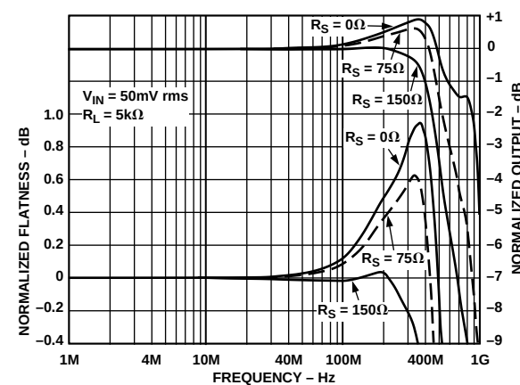
Figure 20. Frequency Response vs. Input Series Resistance
