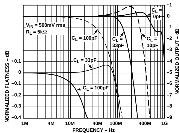
Figure 19. Frequency Response vs. Capacitive Load
