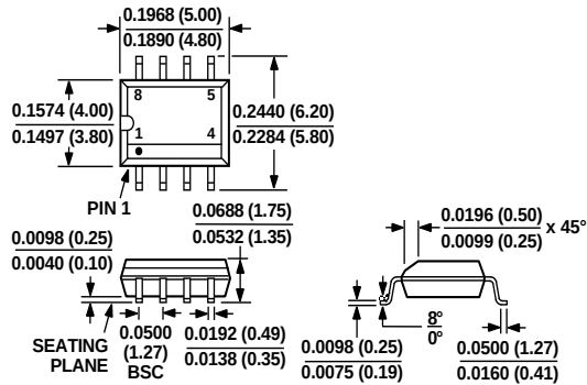
8-Lead Plastic SOIC (SO-8)
