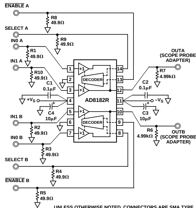
Figure 27. AD8182R Evaluation Board
