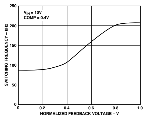
Figure 15. Frequency Foldback
