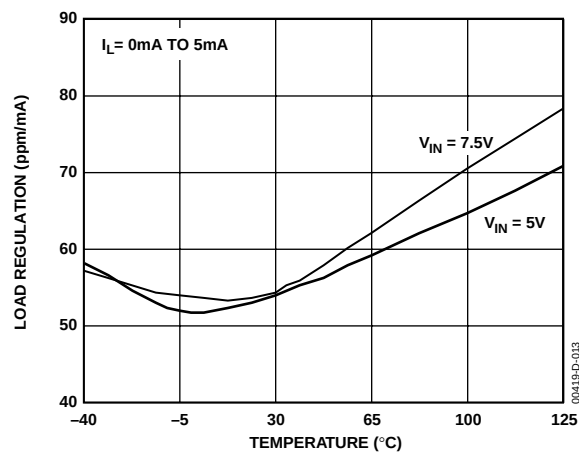
Figure 13. ADR392 Load Regulation vs. Temperature
