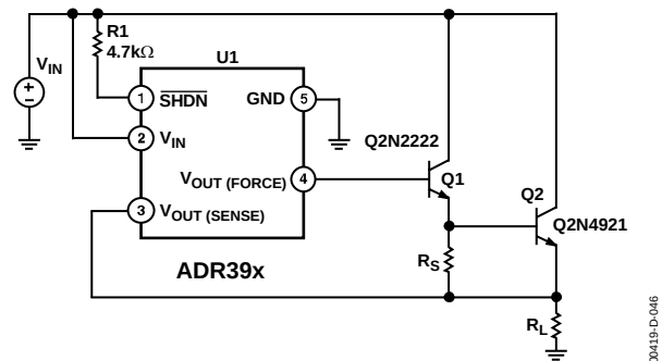
Figure 46. ADR39x for High Output Current with Darlington Drive Configuration
