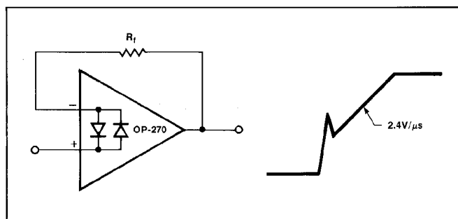
FIGURE 9: Pulsed Operation
