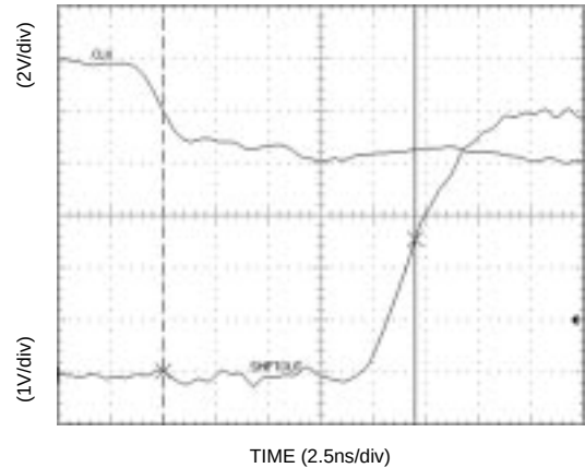
Clock to Shiftout Delay Time
