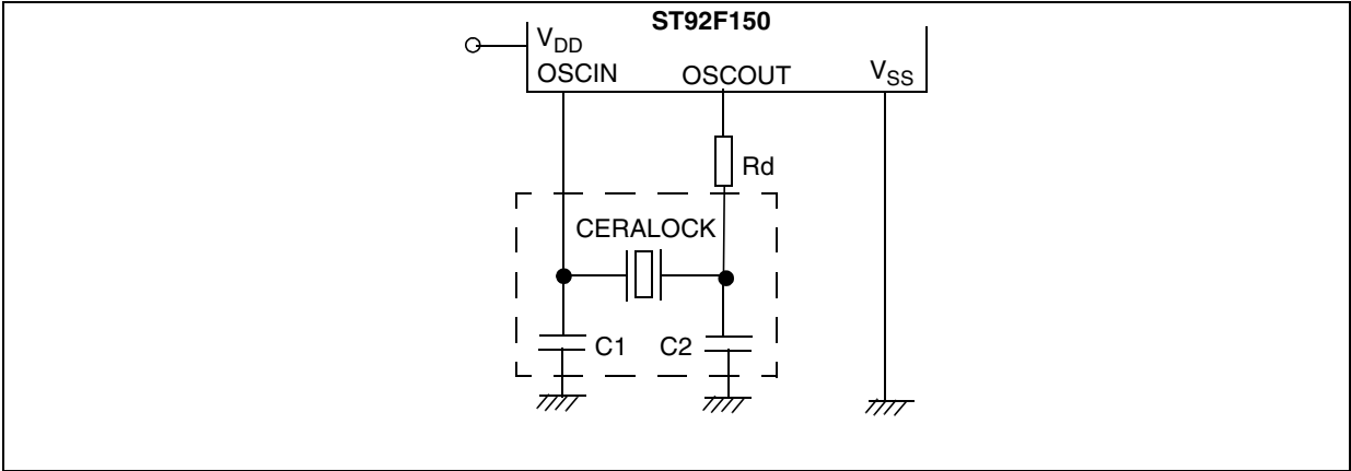
Figure 69. Test Circuit
