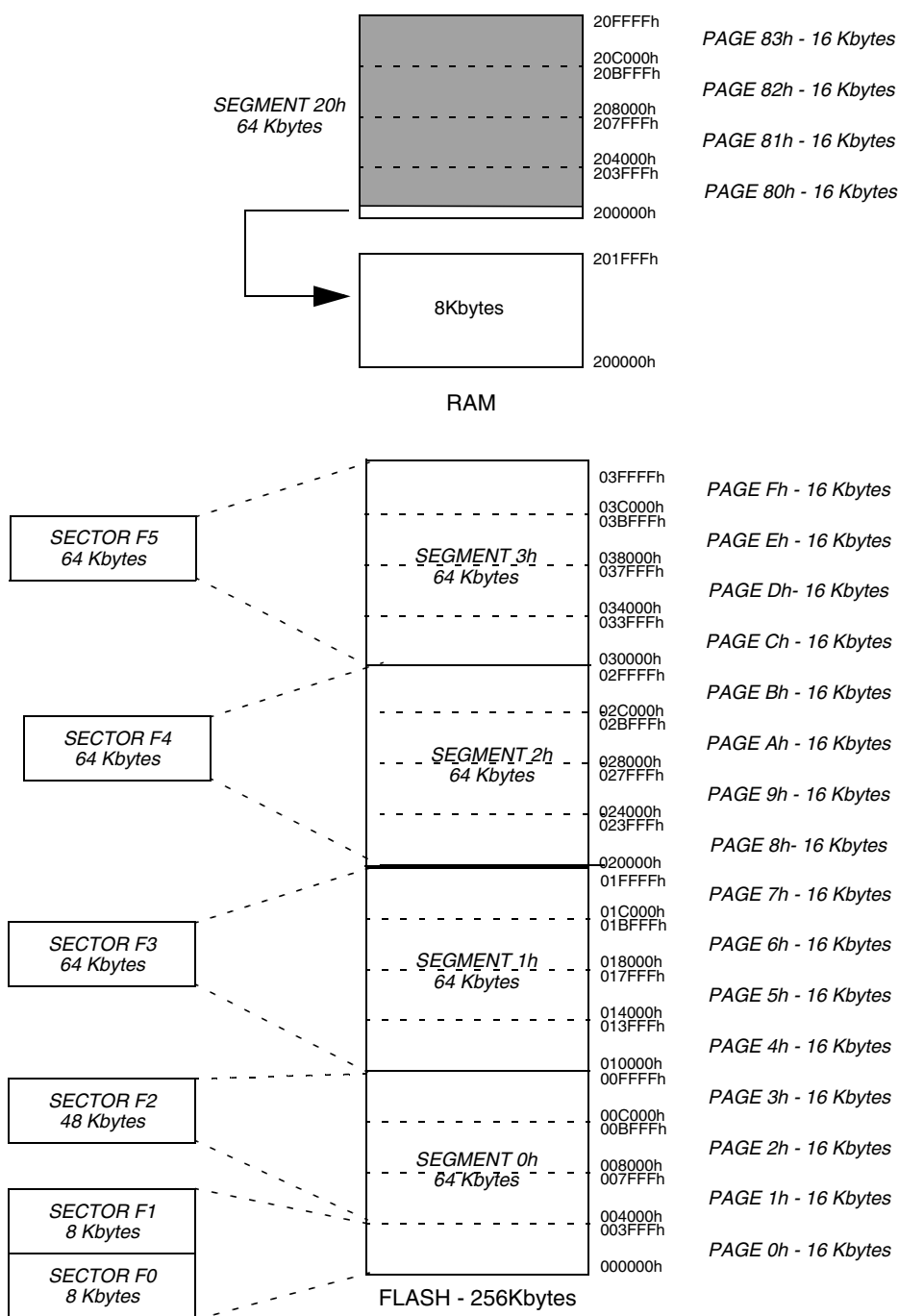
Figure 43. ST92F250 Internal Memory Map (256K version)
