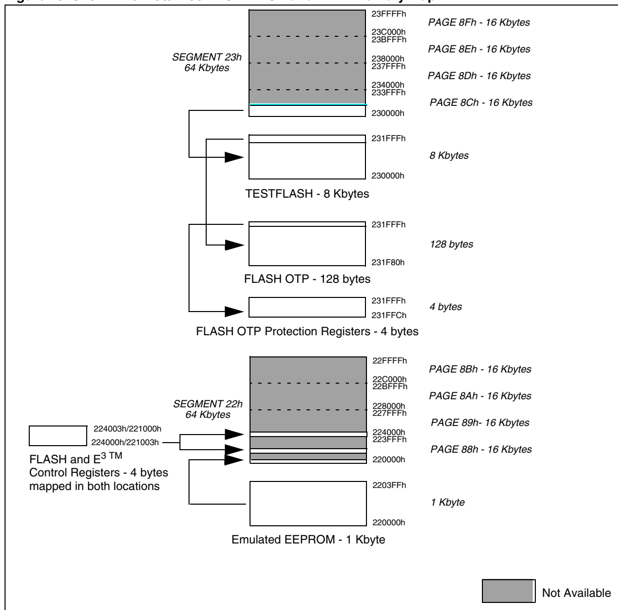
Figure 40. ST92F124/F150/F250 TESTFLASH and E 3 ™ Memory Map
