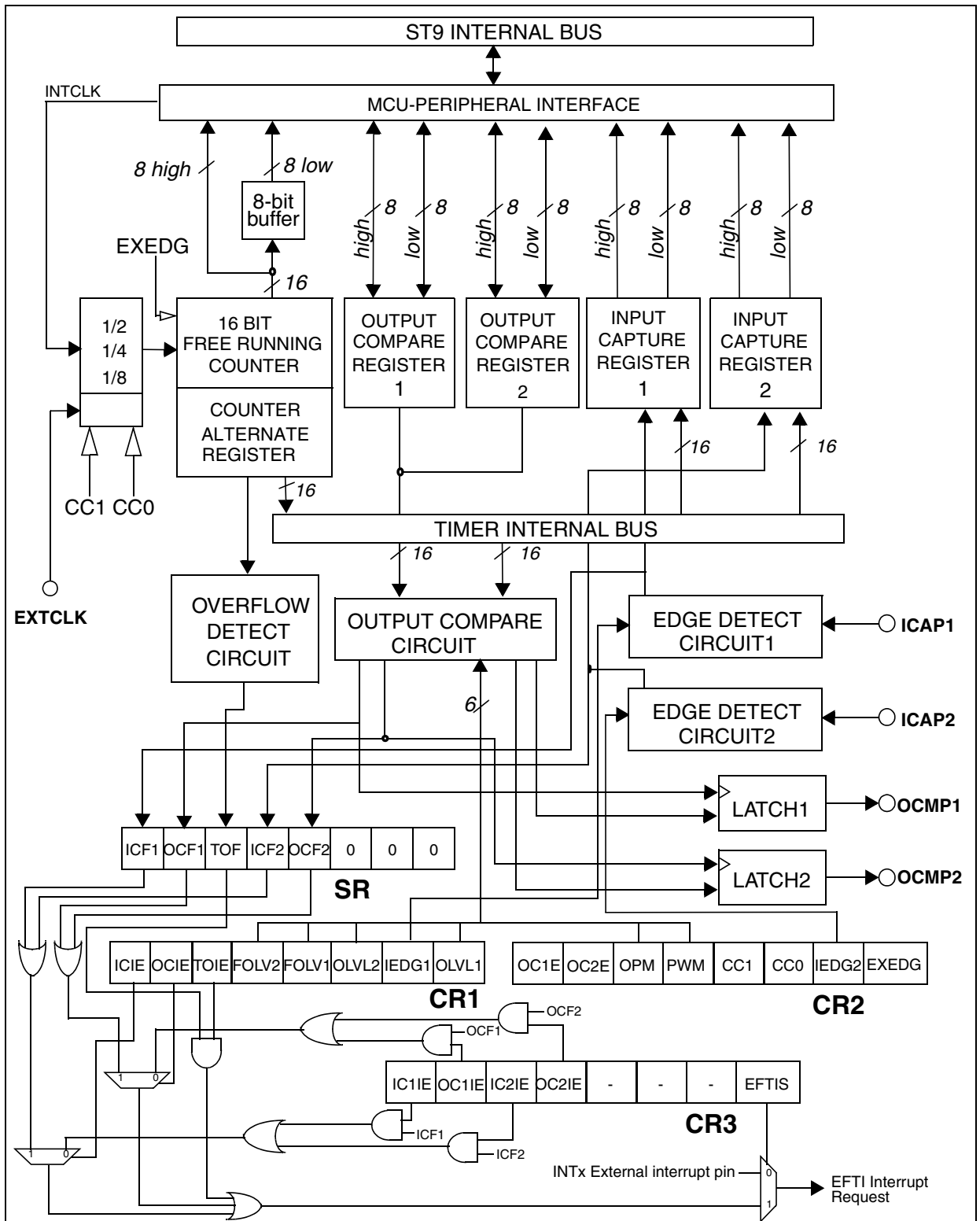
Figure 91. Timer Block Diagram
