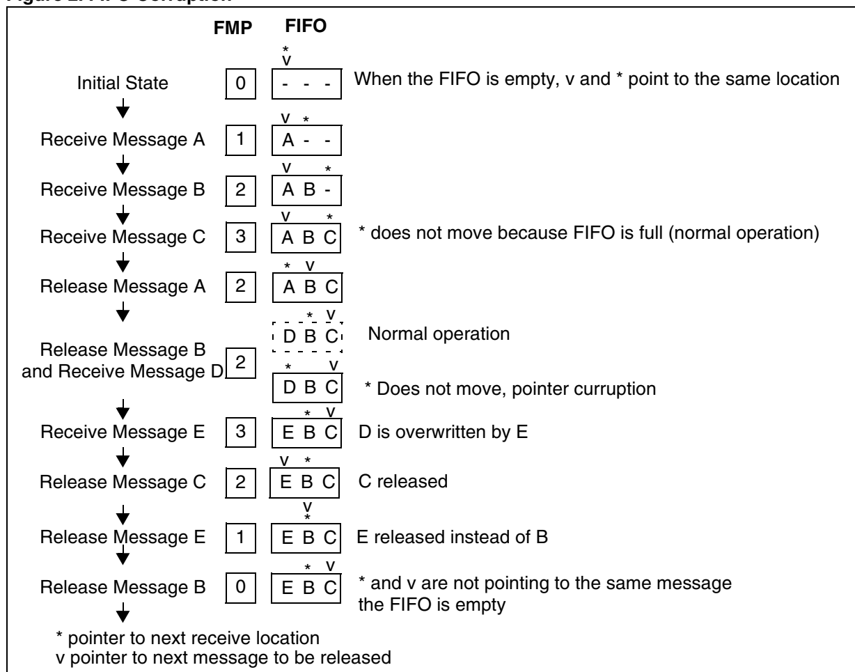
Figure 2. FIFO Corruption
