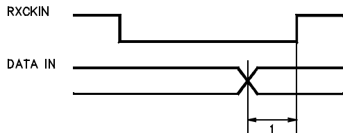
FIG 1: RECEPTION WITH EXTERNAL CLOCK 1X MODE
