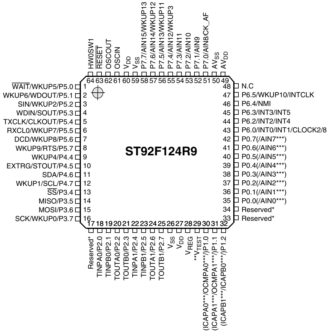
Figure 6. ST92F124R9: Pin Configuration (Top-view TQFP64)
