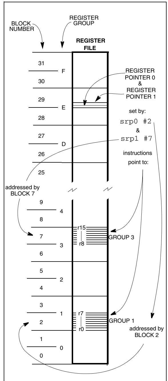
Figure 23. Pointing to two groups of 8 registers
