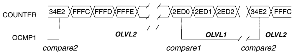
Figure 100. Pulse Width Modulation Mode Timing
