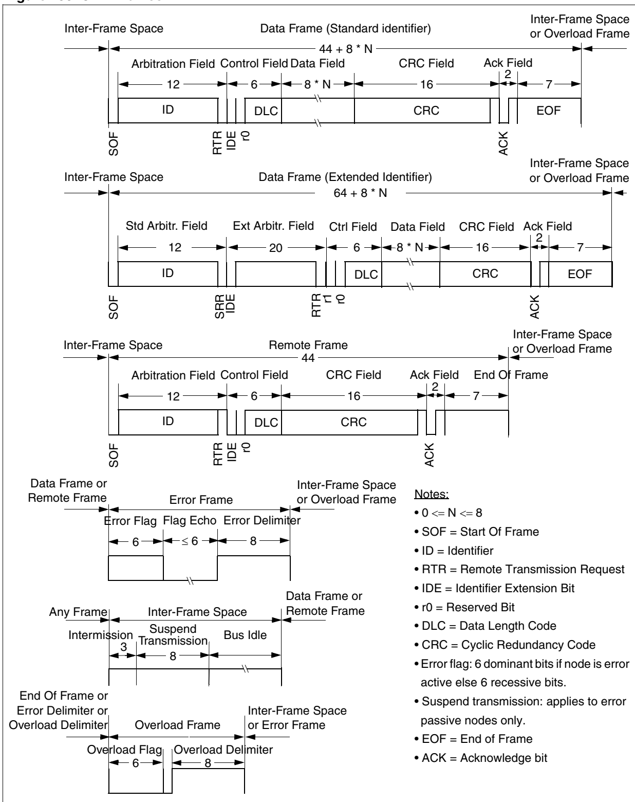
Figure 153. CAN Frames
