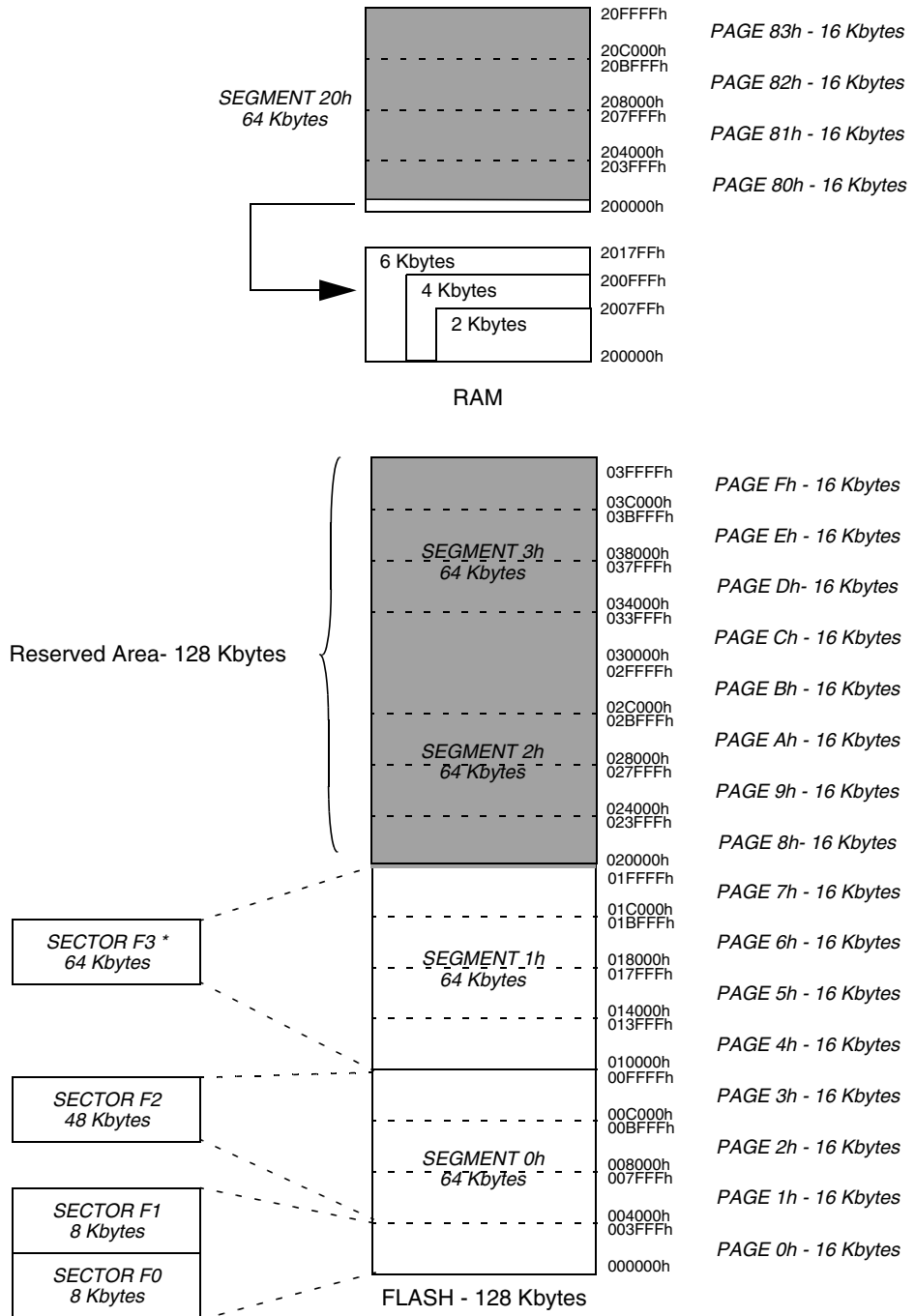
Figure 42. ST92F124/F150 Internal Memory Map (128K versions)
