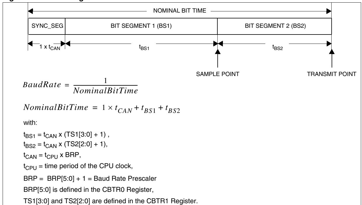
Figure 152. Bit Timing
