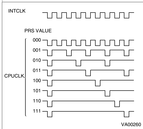
Figure 62. CPU Clock Prescaling
