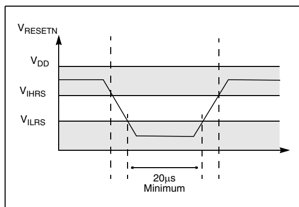
Figure 71. Recommended Signal to be Applied on Reset Pin
