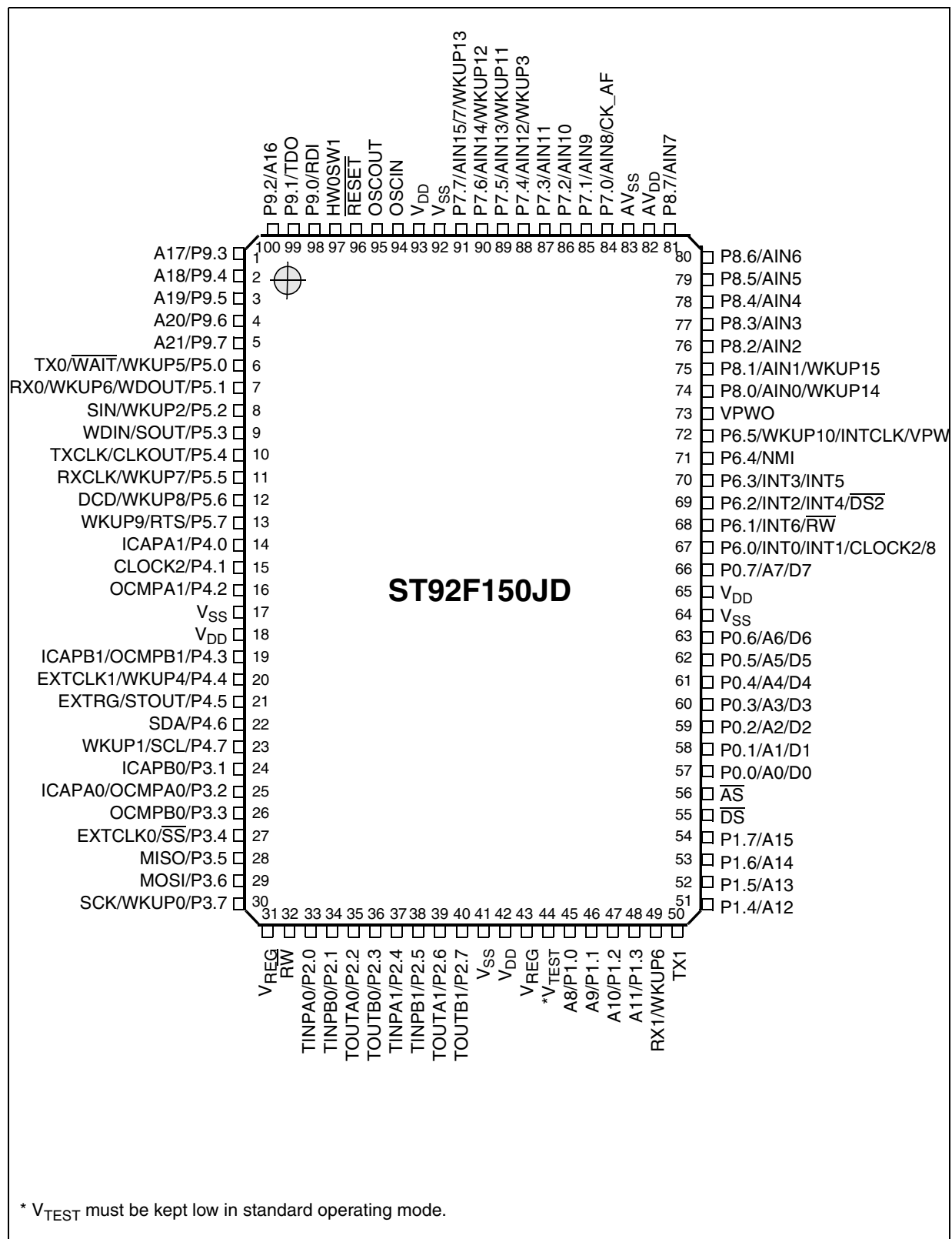
Figure 11. ST92F150JD: Pin Configuration (Top-view PQFP100)
