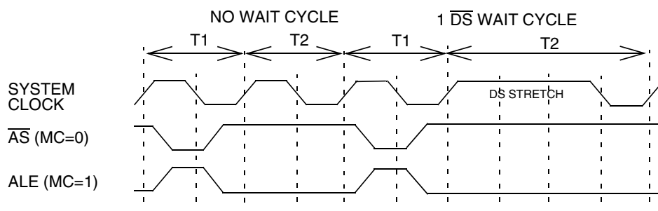
Figure 77. Effects of DS2EN on the behavior of \overline{DS} and \overline{DS2}
