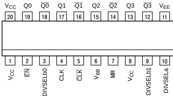
Figure 1. 20-Lead Pinout (Top View)
