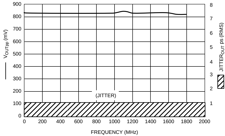
Figure 6. \div 5, F_{max}/Jitter
