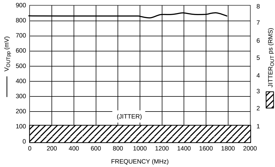
Figure 5. \div 2, F_{max}/Jitter
