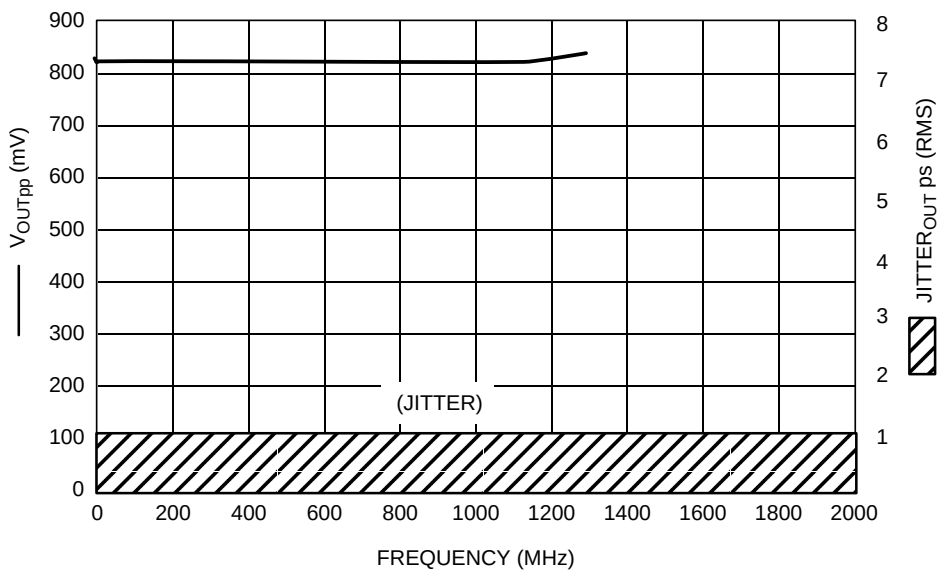
Figure 7. \div 4 , F_{max}/Jitter
