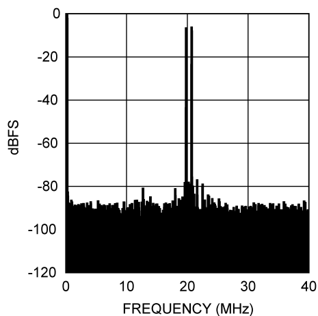
Intermodulation Distortion, f_{IN1} = 19.6 MHz, f_{IN2} = 20.5 MHz
