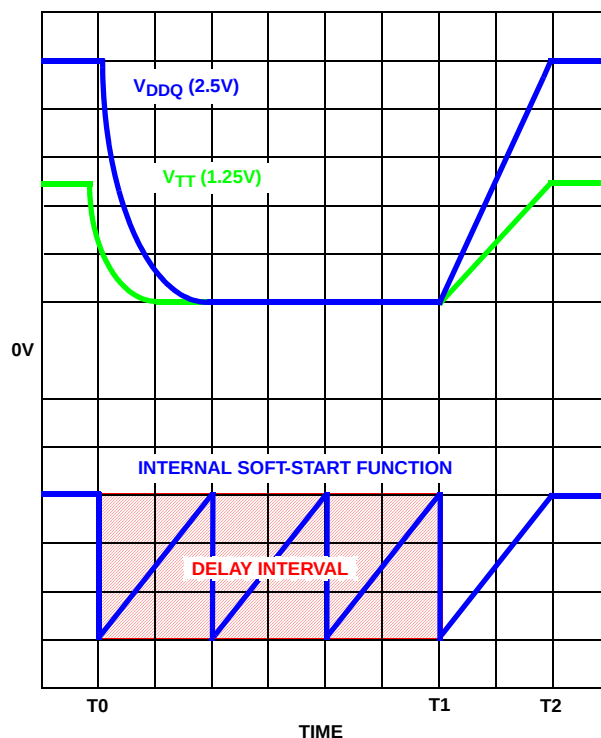
FIGURE 5. OVERCURRENT PROTECTION RESPONSE
