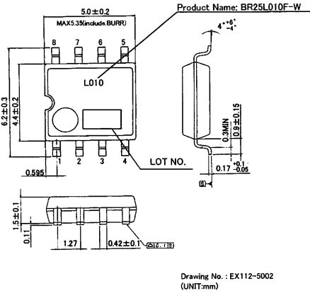
Fig4-(a) PHYSICAL DIMENSION SOP8 (BR25L010F-W)
