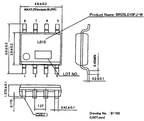
Fig4-(b) PHYSICAL DIMENSION SOP-J8 (BR25L010FJ-W)
