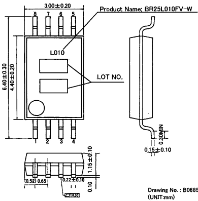
Fig4-(c) PHYSICAL DIMENSION SSOP-B8 (BR25L010FV-W)
