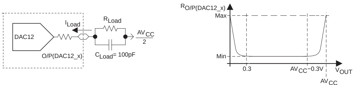
Figure 15. DAC12_x Output Resistance Tests
