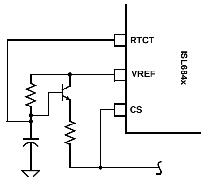
FIGURE 7. SLOPE COMPENSATION
