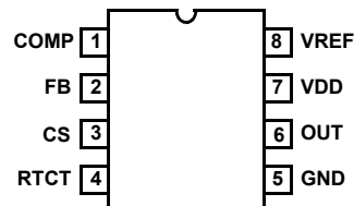
DFN 8 LEAD TOP VIEW
