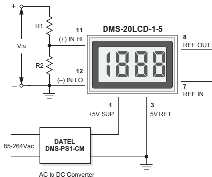
Figure 4. Input Attenuation Circuit
