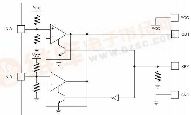
BLOCK DIAGRAM
