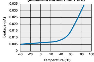
TS190 Typical Leakage vs. Temperature (Measured across Pins 7 & 8)
