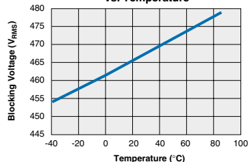
TS190 Typical Blocking Voltage vs. Temperature
