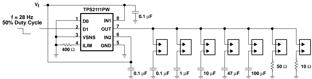
Output Swicthover Voltage Droop Test Circuit
