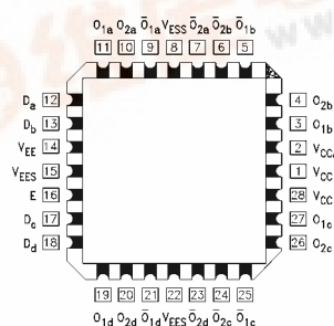
28-Pin PLCC
