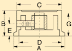
Brass Bushing w/ Set Screw
